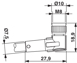
Dimensioned drawing
